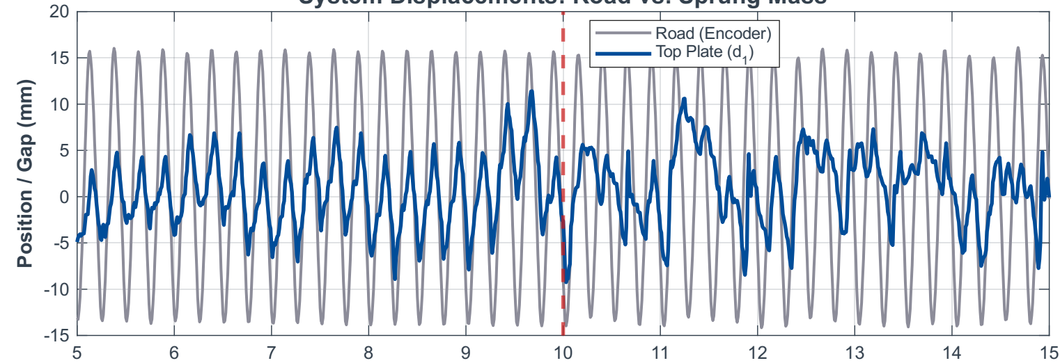
System Displacements: Road vs. Sprung Mass
