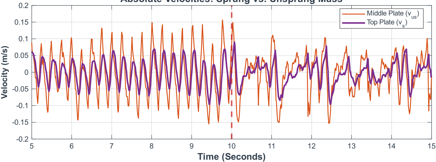
Absolute Velocities: Sprung vs. Unsprung Mass
